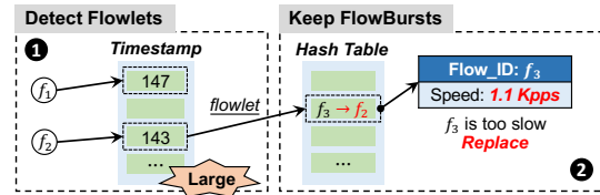
Fig. 1: A strawman solution to detect FlowBursts ( \delta=5\text{ms} , t_{now}=150\text{ms} , \mathcal{V}=1.5\text{Kpps} ).
